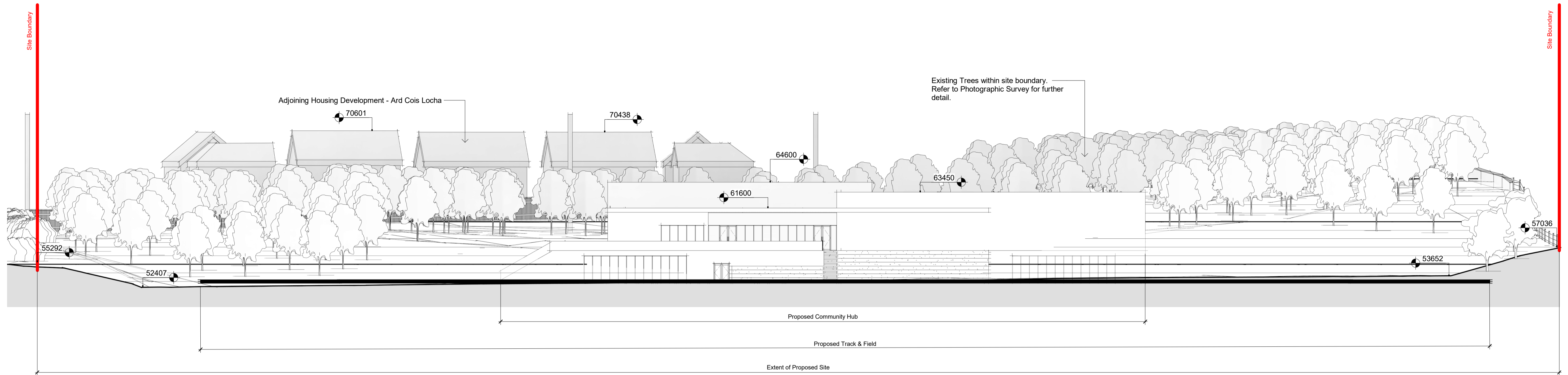
Proposed Site Section BB 1 : 250
